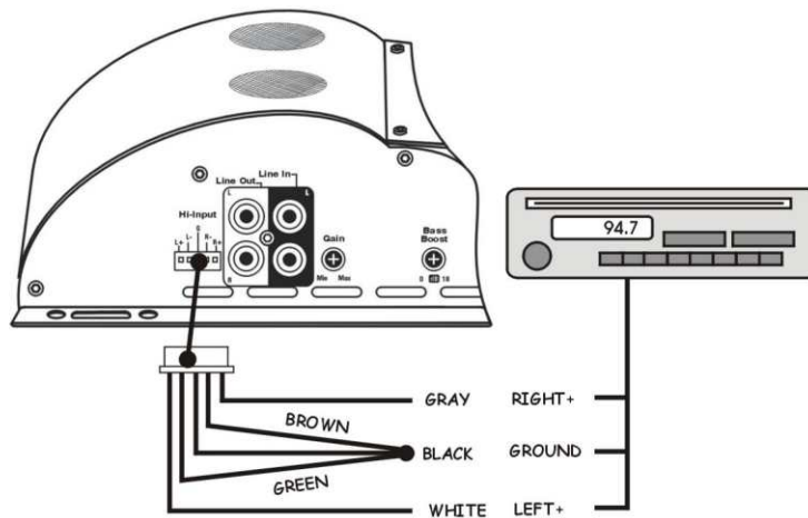
TWO CHANNEL CONNECTIONS: COMMON GROUND RADIO
